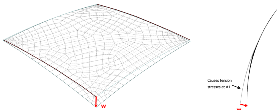
Fig. 20 Deformation due to imposed loads as applied within finite element calculation.
