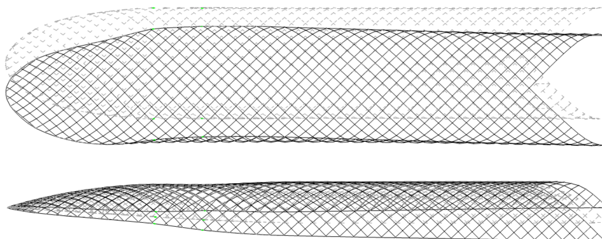
Fig. 11 Horizontal (top) and vertical (bottom) deformation of supporting sub-structure under wind-load conditions.
