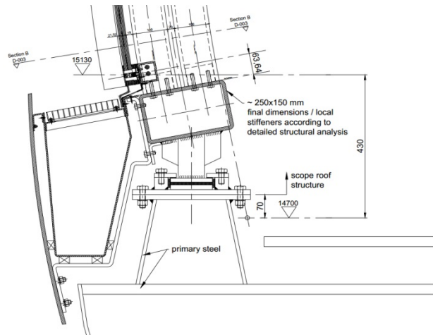
Fig. 16 Typical bearing detail (section and elevation).
