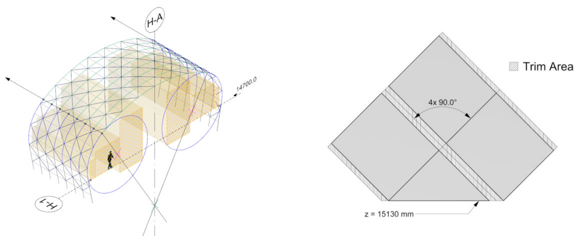
Fig. 7 Generic cross section with diamond pattern (left) / two-side supported glass panes with 90^\circ corners in an unrolled condition (right).
