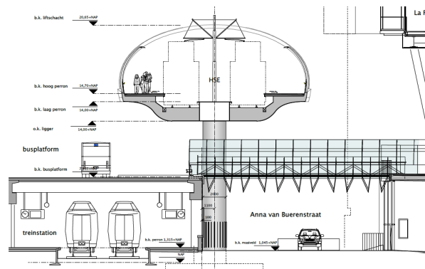
Fig. 1 Cross section – positioning of the piers.
