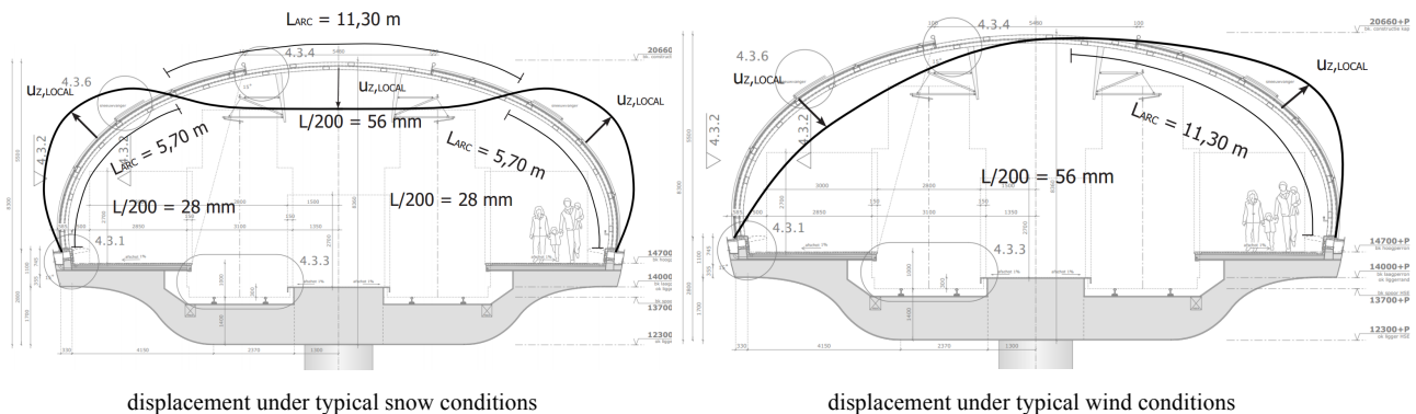
Fig. 18 Typical displacement of roof structure under snow and wind conditions respectively.
