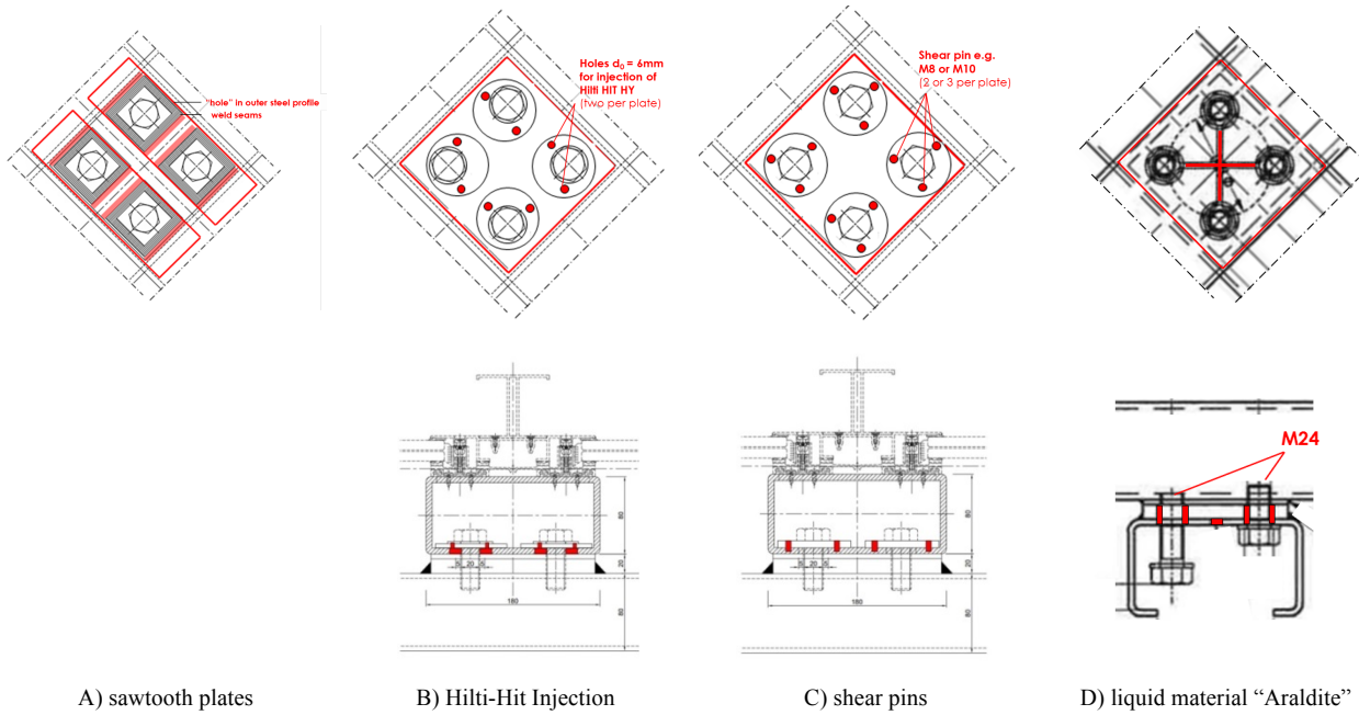
Fig. 14 Options for bolted connection.
