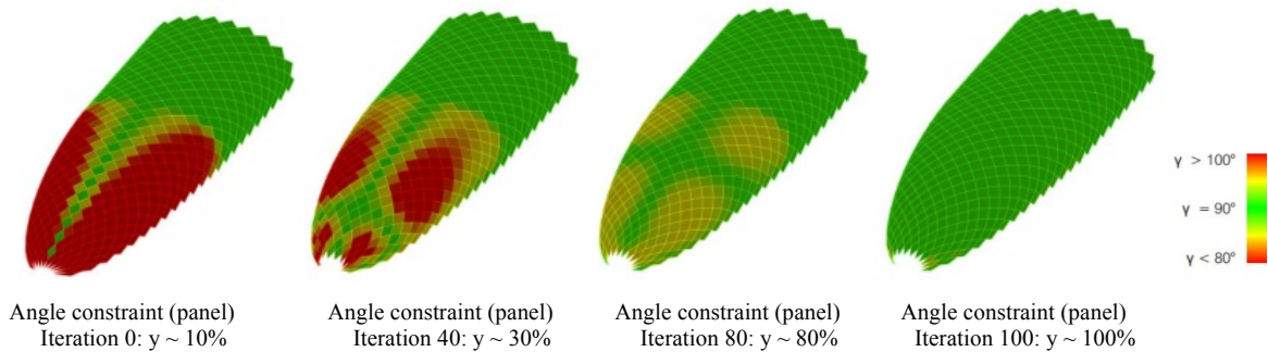
Fig. 8 Optimization of grid in the doubly-curved part.
