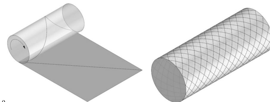
Fig. 6: General principle behind glass and steel geometry.
