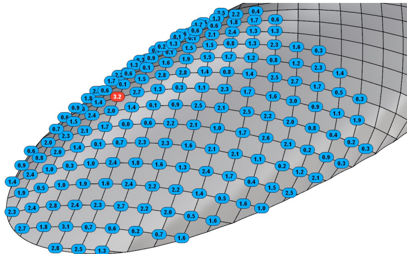
Fig. 9 Distance between glass and steel geometry (mm).
