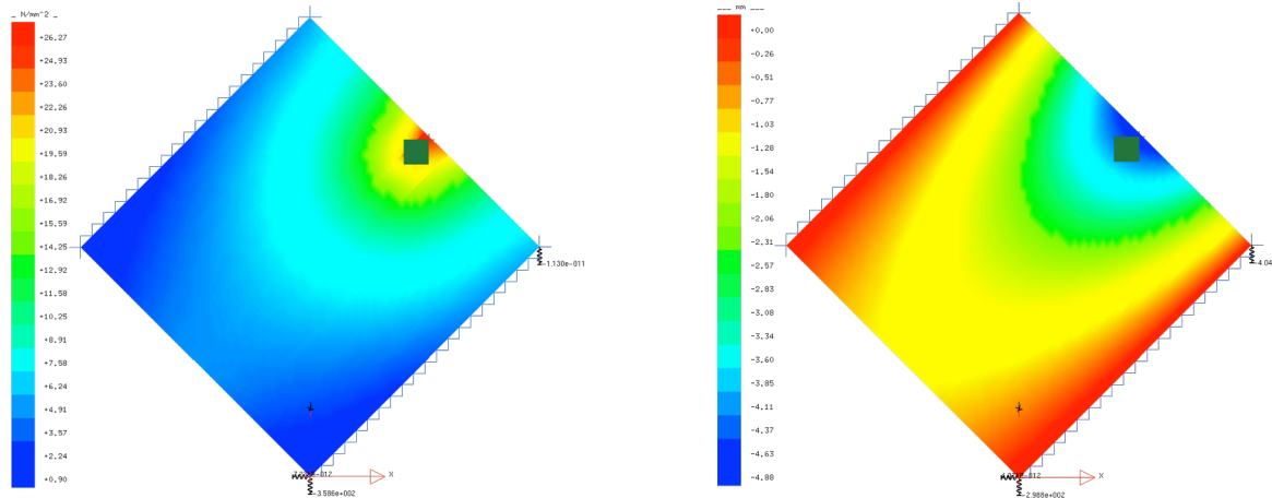
Fig. 21 Max. stresses (left) and deformations (right) for glass type 1 under governing load conditions.
