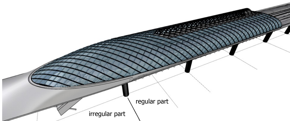
Fig. 5: Roof geometry consisting of irregular (doubly-curved) and regular (generic) part.
