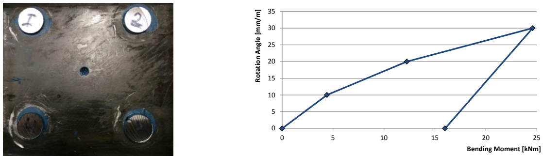
Fig. 15 Bolted connection, oversized holes filled with 'Araldite' (left) and load-deflection behaviour (right).
