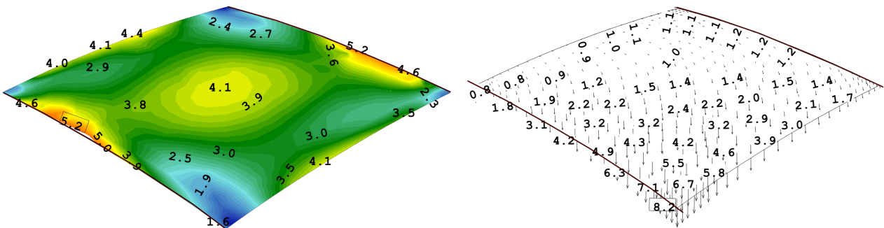
Fig. 22 Maximum tension stress [N/mm 2 ] (left) and deformation [mm] (right) – long-term / permanent load character (LCD 1).
